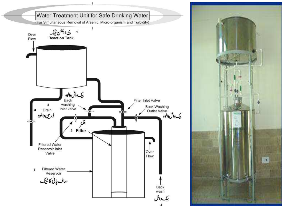
Figure 6. Schematic view of 300 liters arsenic removal unit (ART), showing various components
